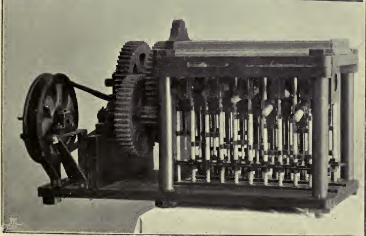
POWDER-MACHINES.
